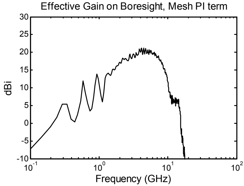
Figure 6.5. The effective gain of the mesh prototype on boresight, with feed arms terminated in 185-ohm resistors.
