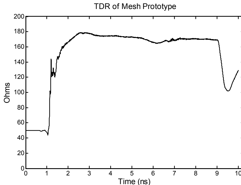
Figure 6.1. TDR of Mesh Prototype.
