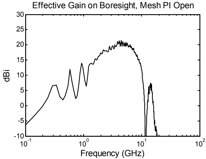
Figure 6.3. The effective gain of the mesh prototype on boresight, with feed arms left open.
