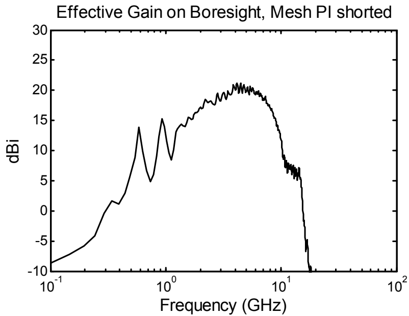
Figure 6.4 The effective gain of the mesh prototype on boresight, with feed arms shorted to the reflector.
