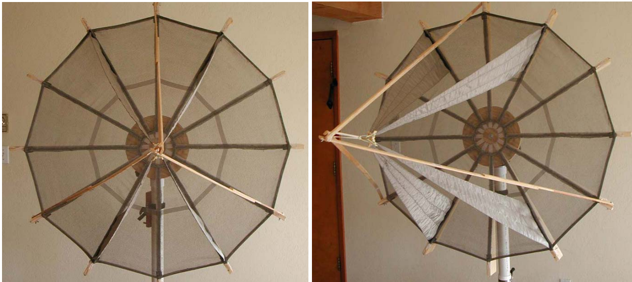
Figure 5.1. Two views of the mesh Para IRA prototype before improved feed point installation.
