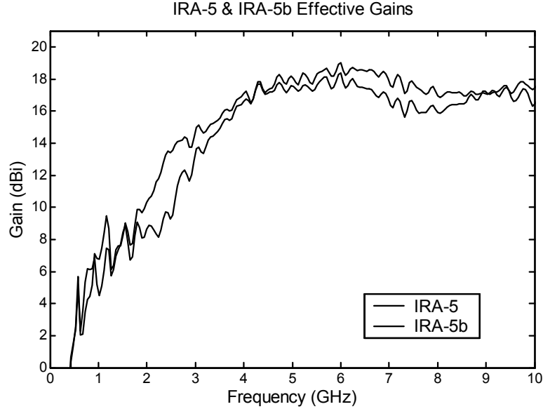
Figure 4.10. Effective gain for IRA-5 and the IRA-5b.
