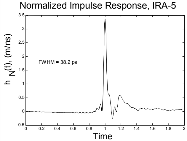
Figure 4.4. Normalized impulse responses in the time domain. (IRA-3 left, IRA-5 right)
