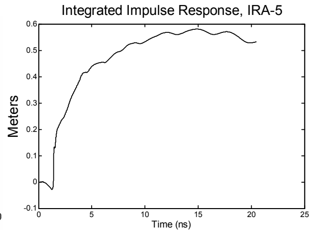
Figure 4.6. Integrated impulse responses in the time domain. (IRA-3 left, IRA-5 right)
