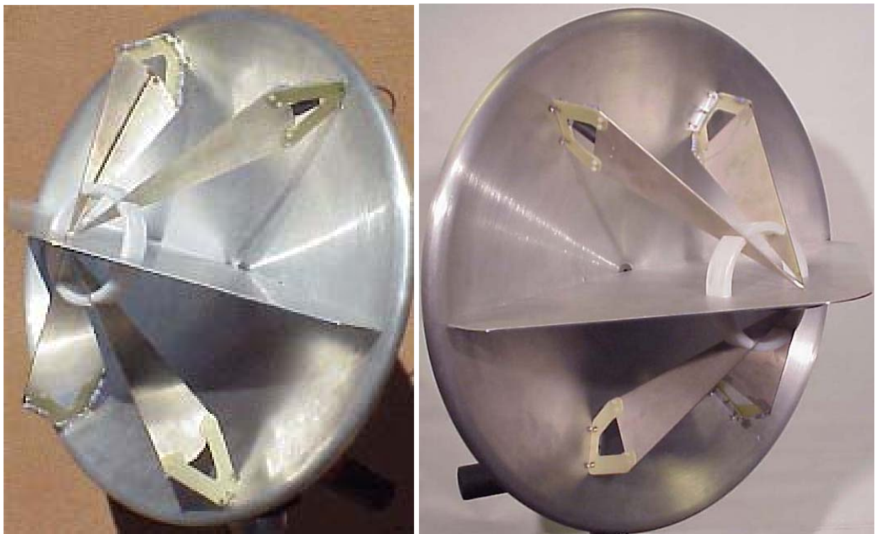
Figure 2.3. The IRA-3 (left) and IRA-4 (right).
