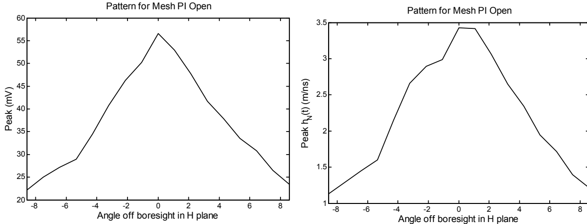
Figure 6.7. H-plane peak raw data and impulse response patterns, with feed arms open.
