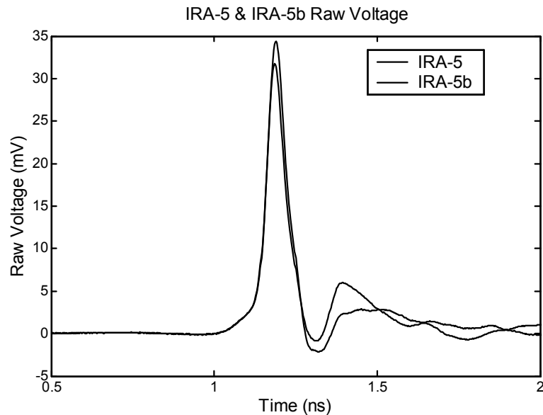
Figure 4.9. Raw voltage for the IRA-5 and IRA-5b.
