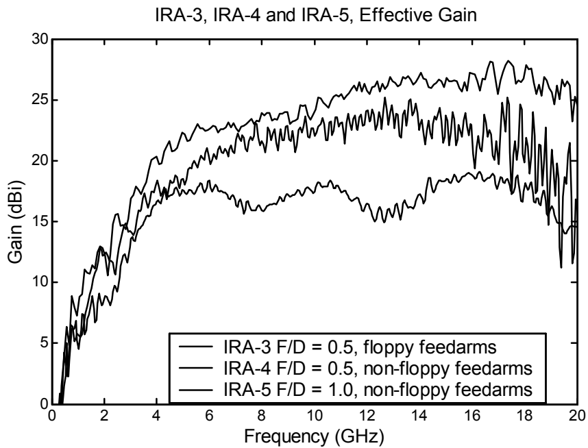
Figure 4.3. Effective gain of the IRA-3, IRA-4 and IRA-5 (top trace to bottom trace, respectively).
