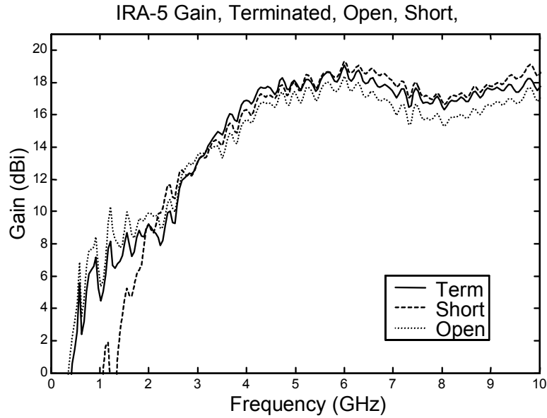
Figure 4.8. Comparison of the effective gain for the three terminations.
