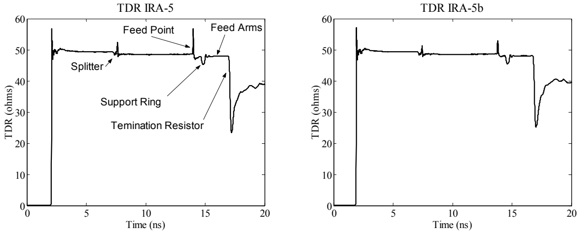
Figure 4.1. Impedance profile of the IRA-5 and IRA-5b.
