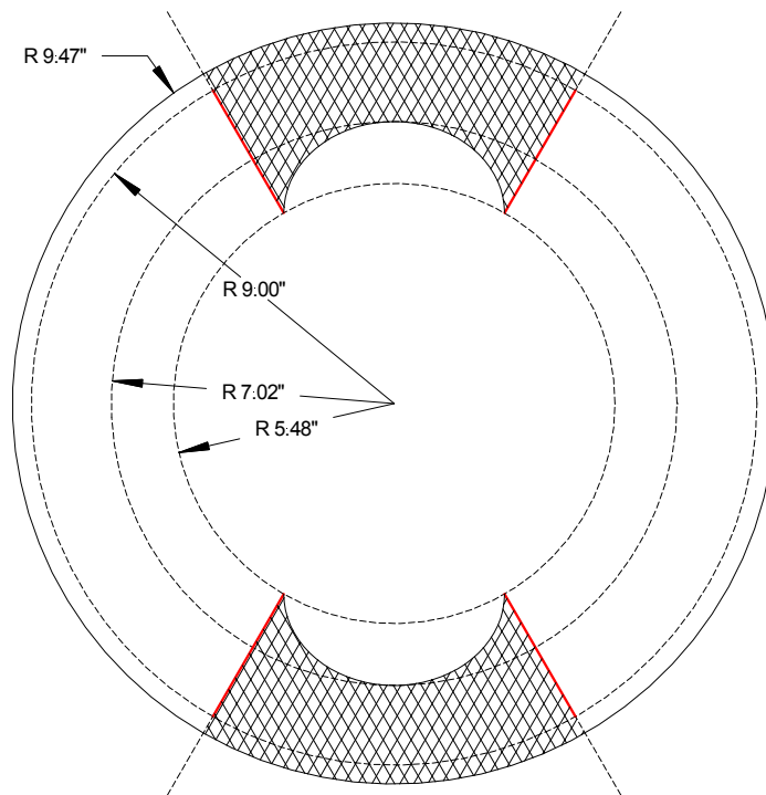
Figure 3-2. Shaped IRA-5 dish with removed area crosshatched.
