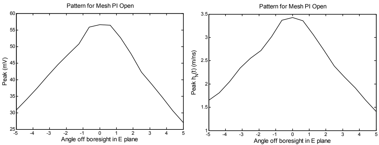
Figure 6.6. E-plane peak raw data and impulse response patterns, with feed arms open.
