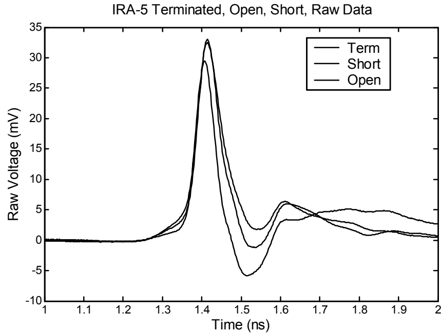
Figure 4.7. Comparison of the raw data for the three terminations.
