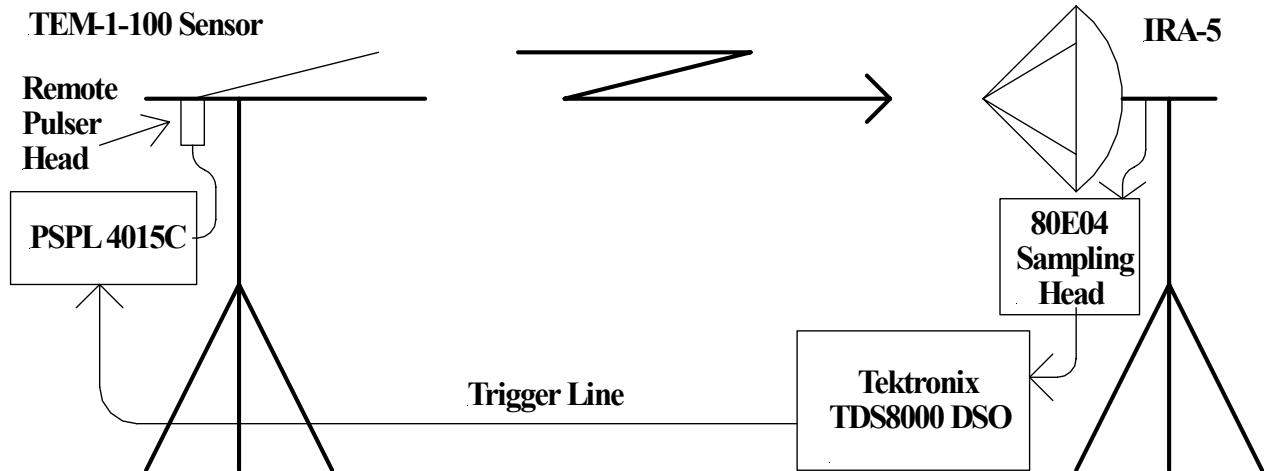
Figure 4.2. Instrumentation setup to measure the response of the IRA-5.
