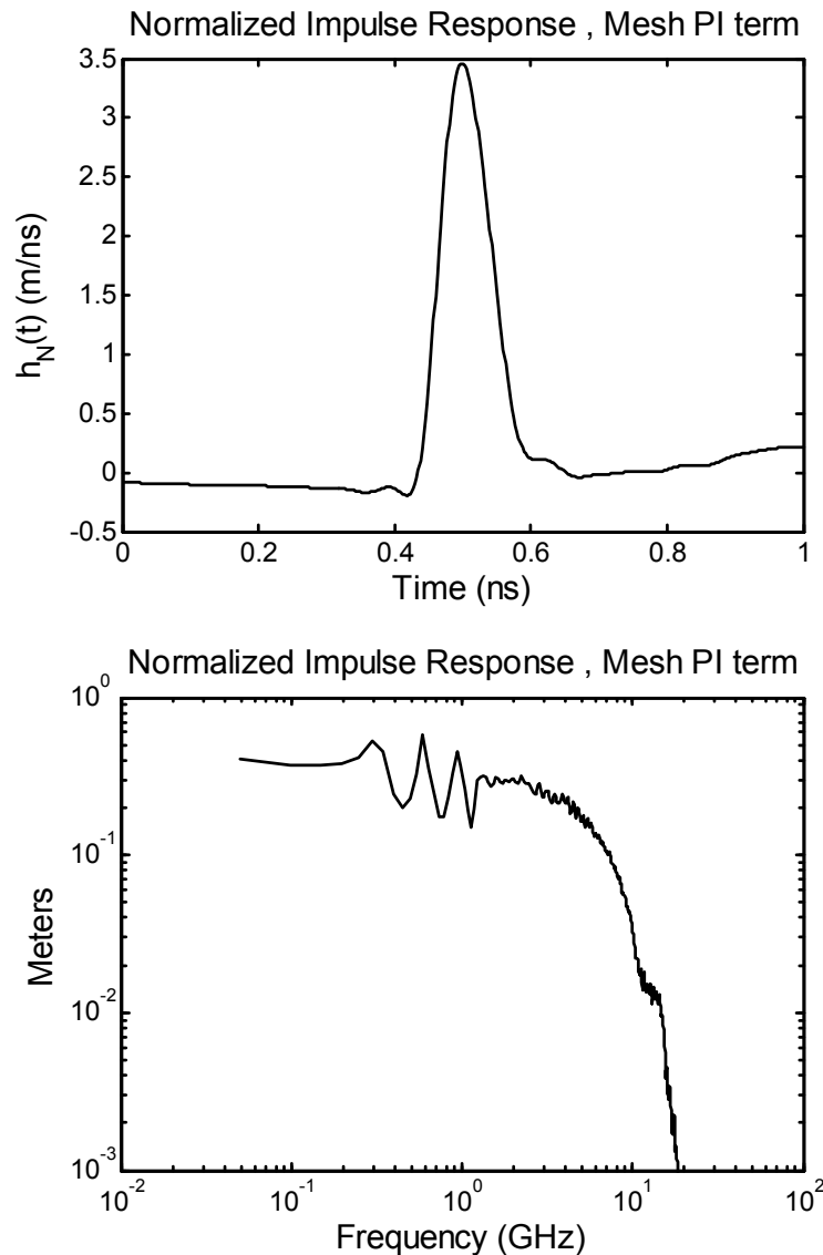
Figure 6.2. The normalized impulse response of the Para-IRA with feed arms terminated in 185 ohms, in both the time domain (top) and in the frequency domain.
