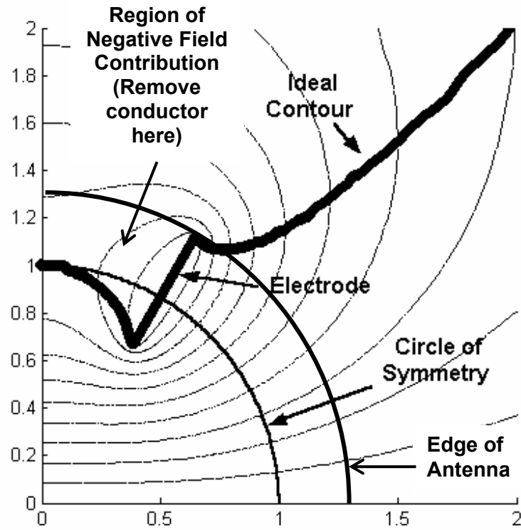
Figure 3.1. Sketch of the aperture fields of one-quarter of an IRA reflector. Note the Region of Negative Field Contribution, where conductor in the reflector should be removed.
