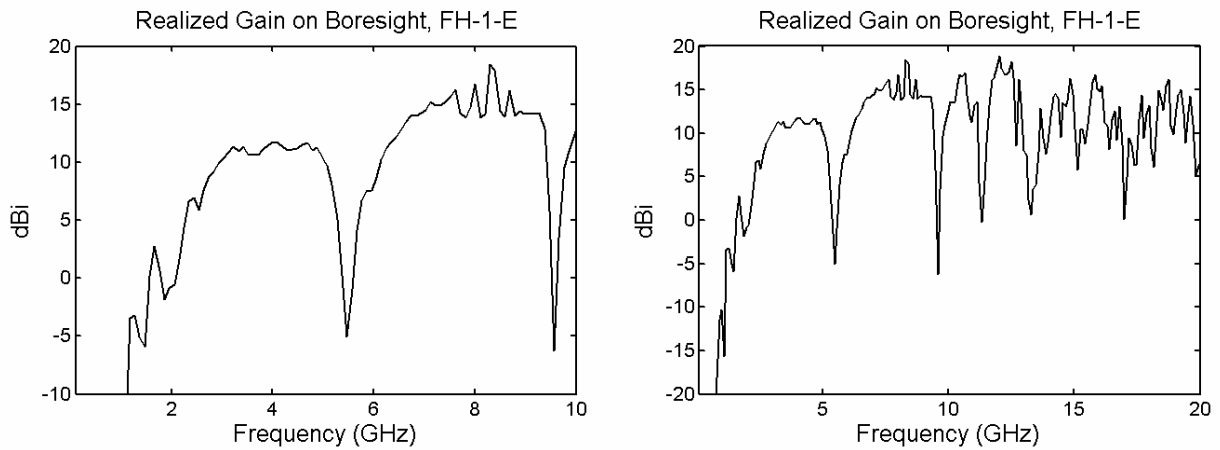
Figure 6.2. Realized gain of the FH-1E with conical feed and Teflon disk.
