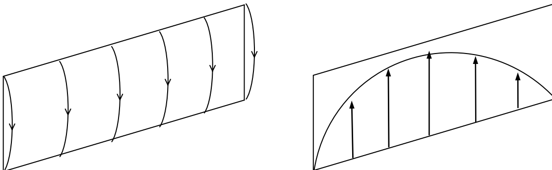
Figure 2.3. Aperture electric fields of the folded horn.
