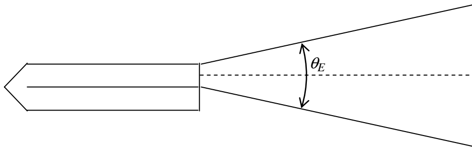
Figure 8.2. Adjusting the opening angle in the E-plane to optimize gain.
