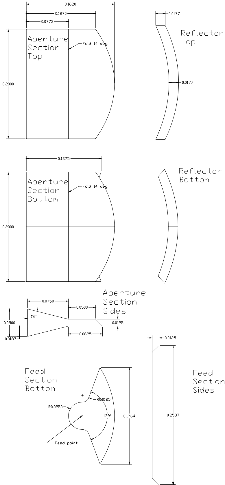
Figure 3.2. Patterns for FH-1 parts. Dimensions are in meters.
