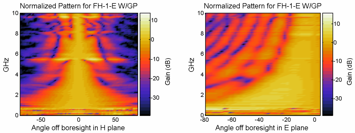
Figure 7.5. Antenna patterns for the FH-1E with ground plane, based on realized gain normalized to boresight.
