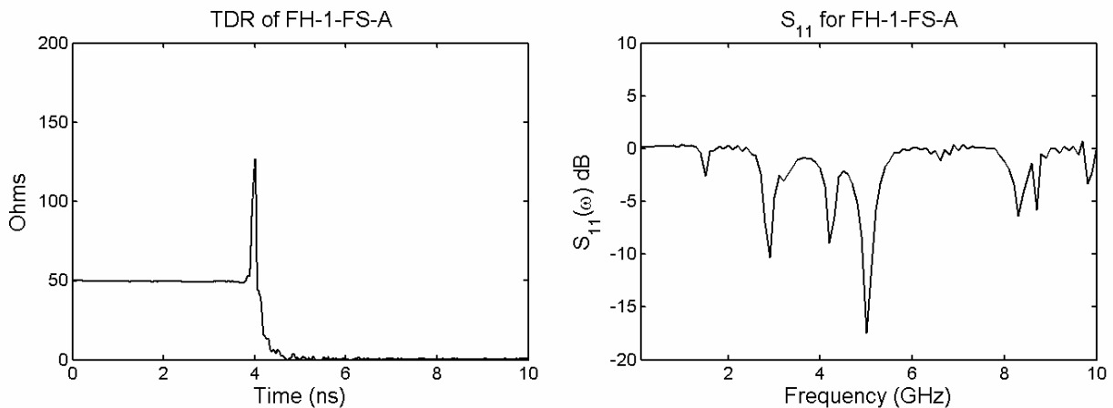
Figure 5.2. TDR and S_{11} of FH-1-FS-A, with Teflon disk.
