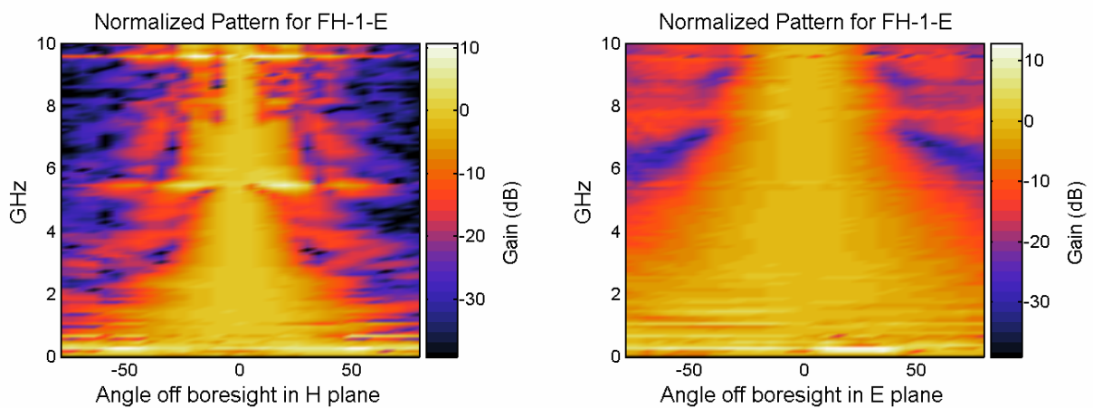
Figure 6.3. Normalized pattern as a function of frequency for the FH-1E, based on realized gain normalized to boresight.
