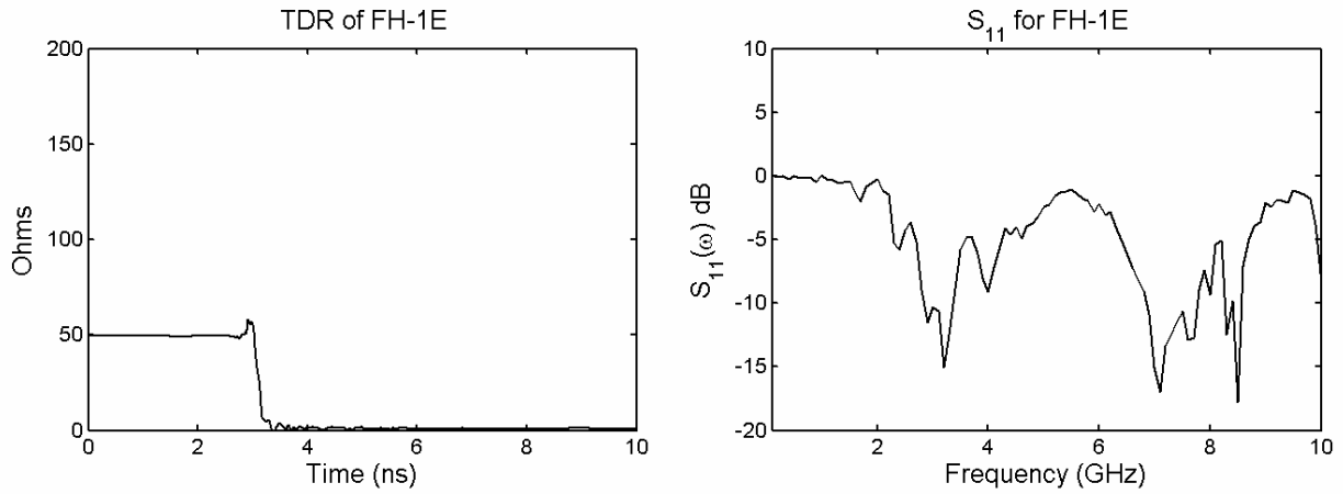
Figure 6.1. TDR and S_{11} of FH-1E with conical feed and Teflon disk.
