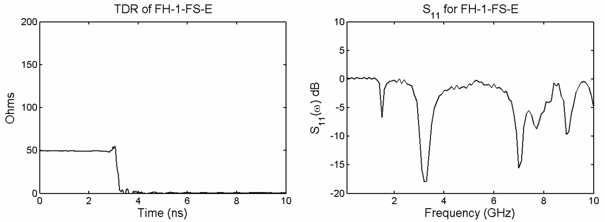
Figure 5.8. TDR and S_{11} of FH-1-FS-E with conical feed and Teflon disk.
