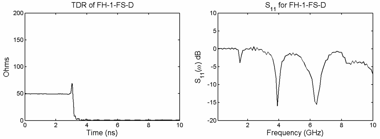
Figure 5.7. TDR and S_{11} of FH-1-FS-D with conical feed.
