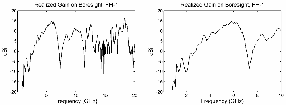
Figure 4.5. Realized Gain of FH-1 folded horn.
