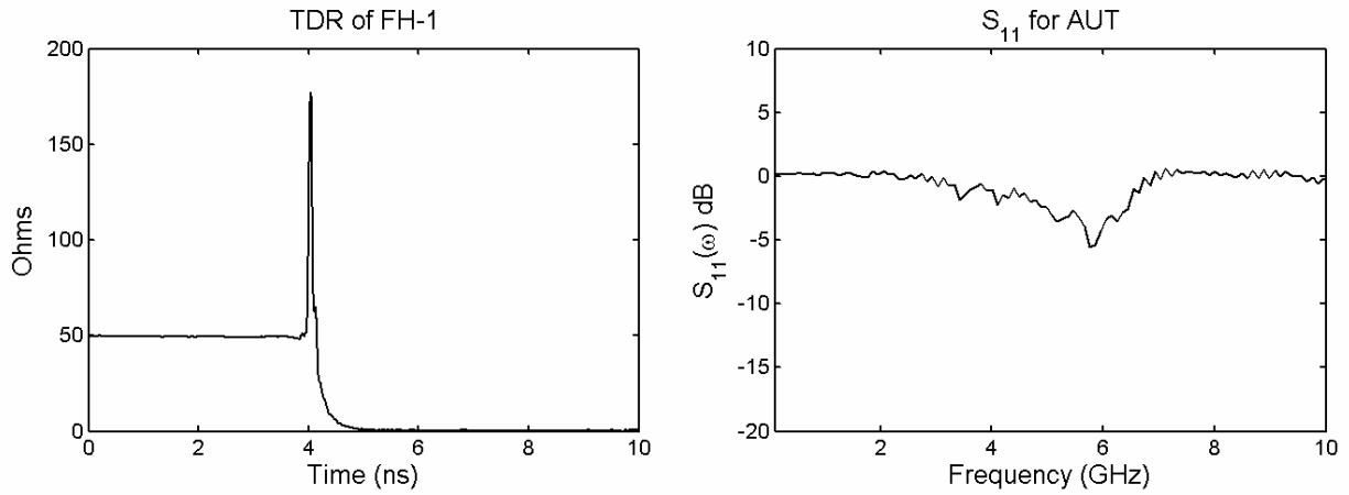
Figure 4.4. TDR and S_{11} of FH-1 folded horn.
