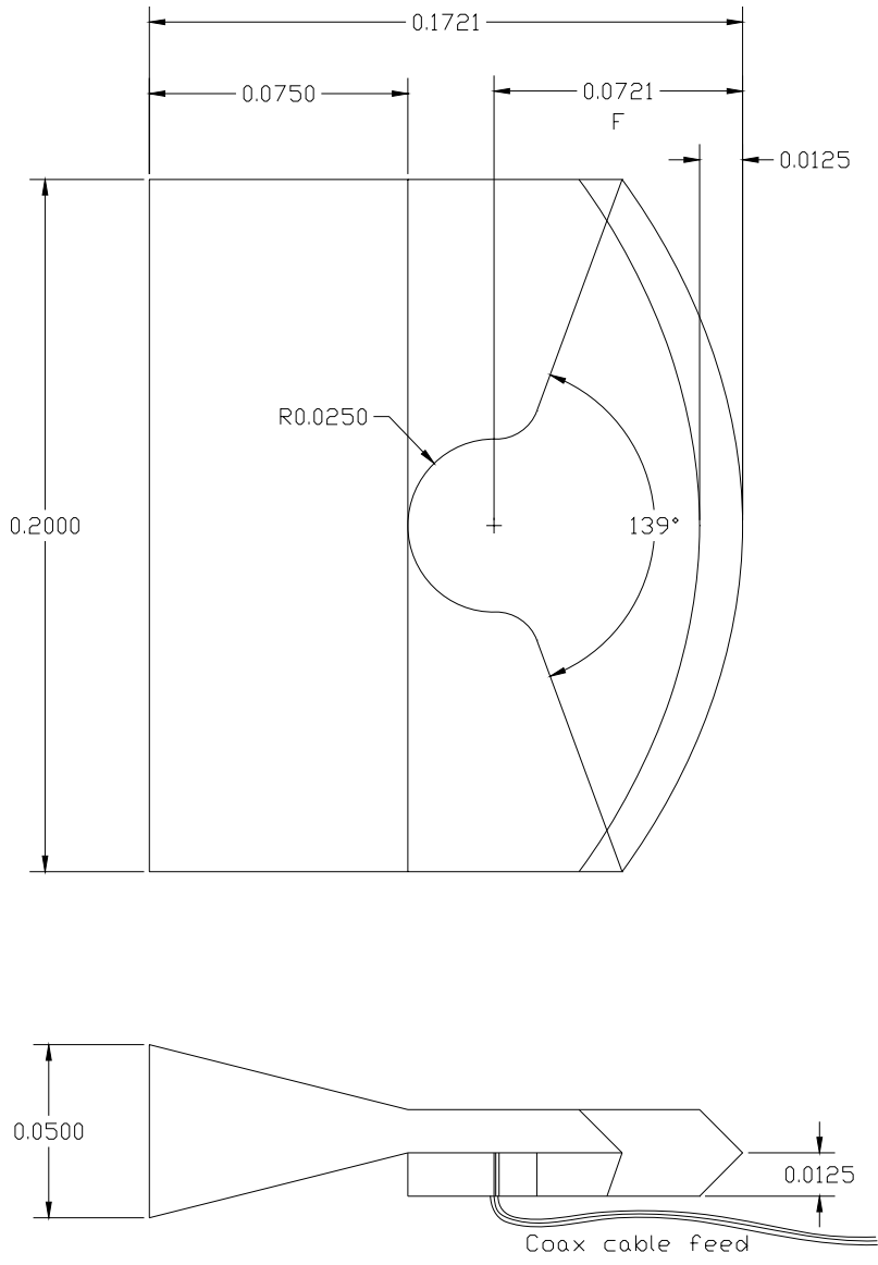
Figure 3.1. FH-1 drawing. Dimensions are in meters.
