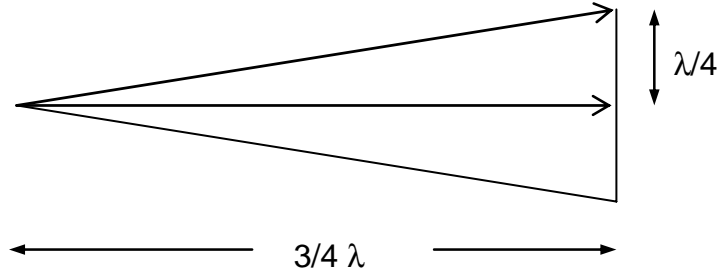
Figure 2.4. Geometry for calculating the level of defocus in the folded horn Aperture section.
